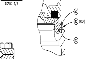
SEAT AND DISC DETAIL SCALE: NONE
