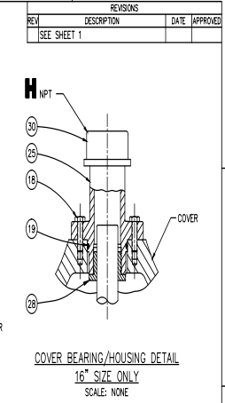
COVER BEARING/HOUSING DETAIL 16" SIZE ONLY SCALE: NONE
