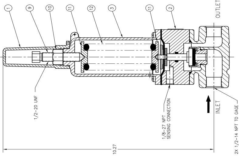
100-300 PSI HIGH PRESSURE DESIGN
